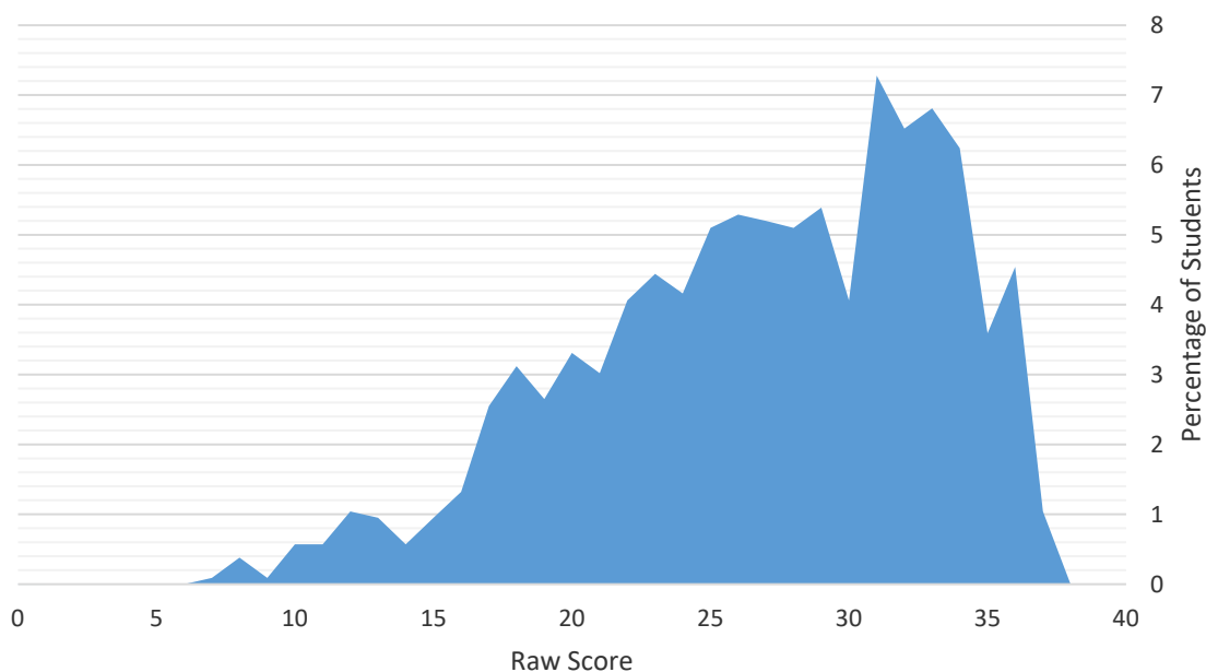
TP26 Part I and II based on the modeled scores of 1075 students from 6 institutions
