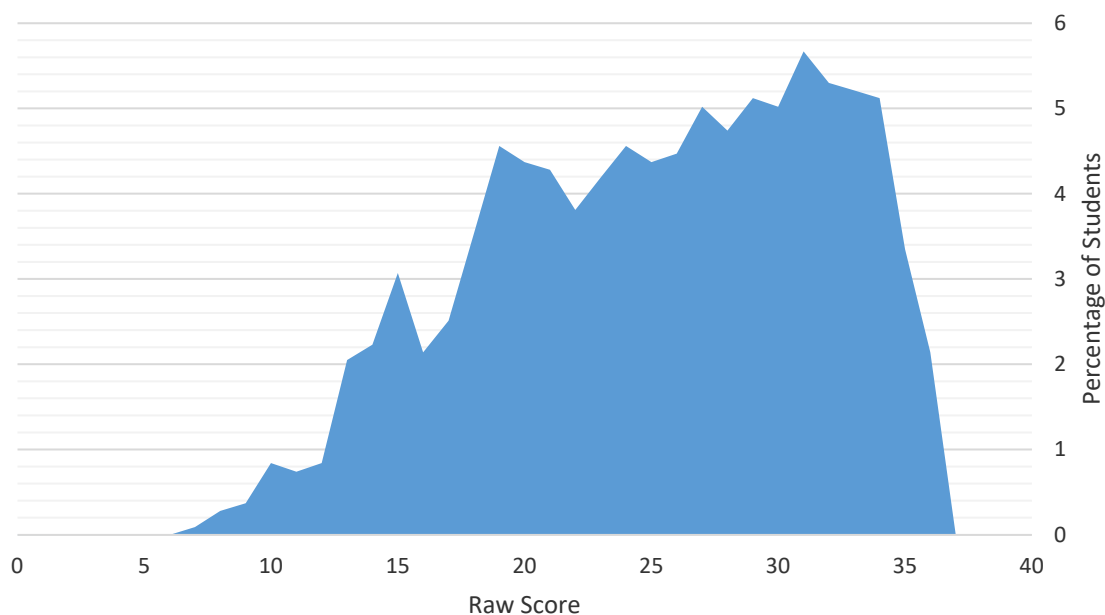
TP26 Part I and III based on the modeled scores of 1075 students from 6 institutions
