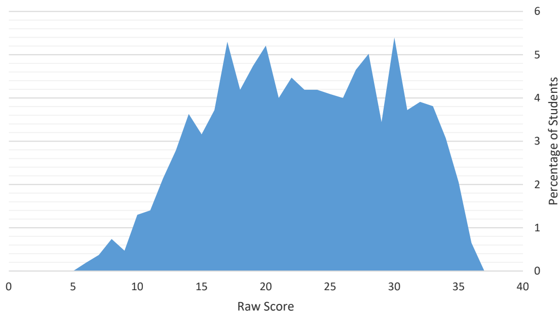
TP26 Part II and III based on the modeled scores of 1075 students from 6 institutions
