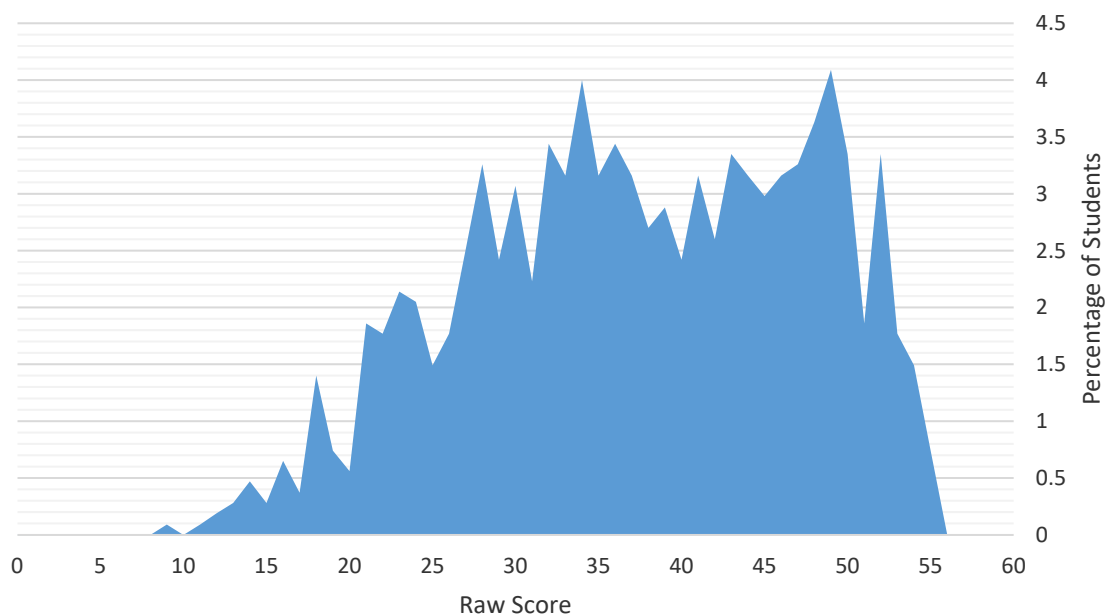
TP26 Part I, II and III based on the modeled scores of 1075 students from 6 institutions
