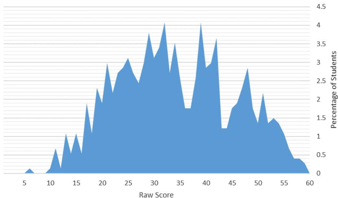
GB14: Organic Chemistry Subtest based on the scores of 737 students from 14 different institutions
