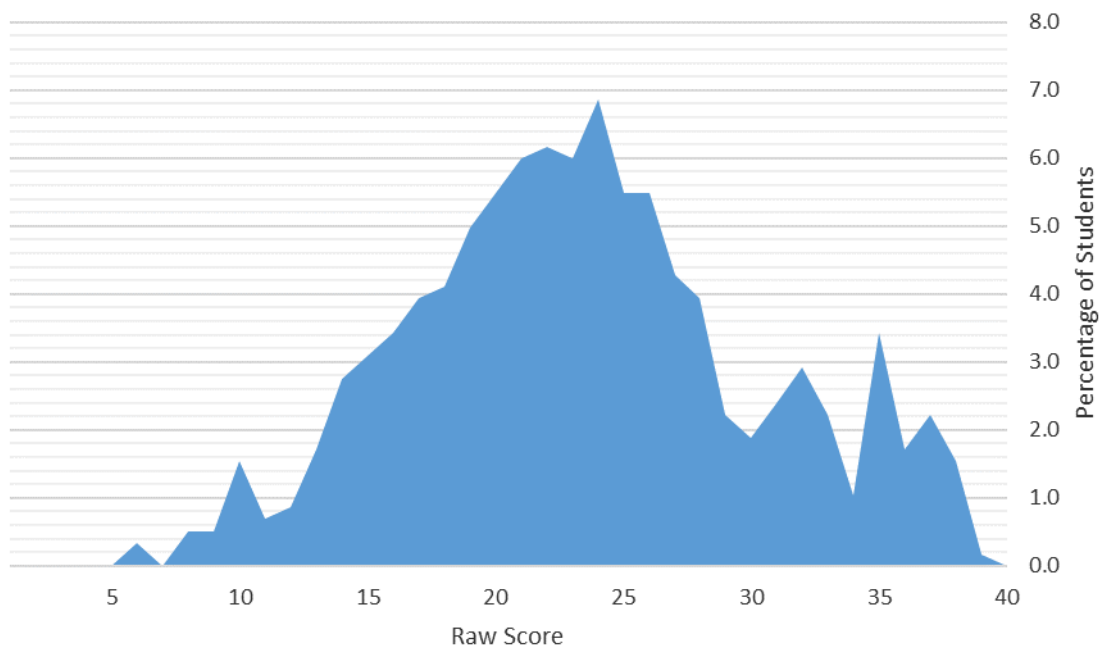
GB14: Organic Chemistry Subtest - Part A based on the scores of 583 students from 8 different institutions
