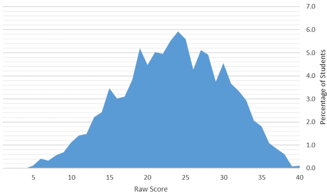
GB14: General Chemistry Subtest - Part A based on the scores of 2483 students from 18 different institutions
