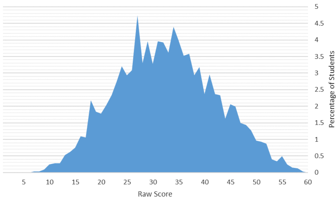
GB14: General Chemistry Subtest based on the scores of 3210 students from 26 different institutions
